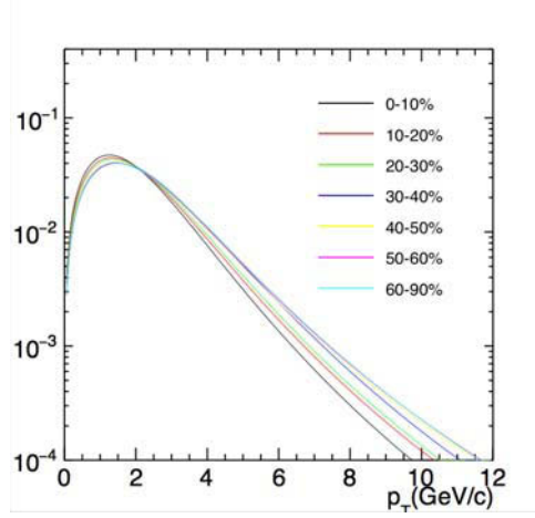
Figure 3.10: Simulated acceptance×efficiency corrected J/\psi p_T distributions in seven centrality bins.
