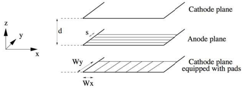
Figure 2.8: Schematic of the CPC [194].
