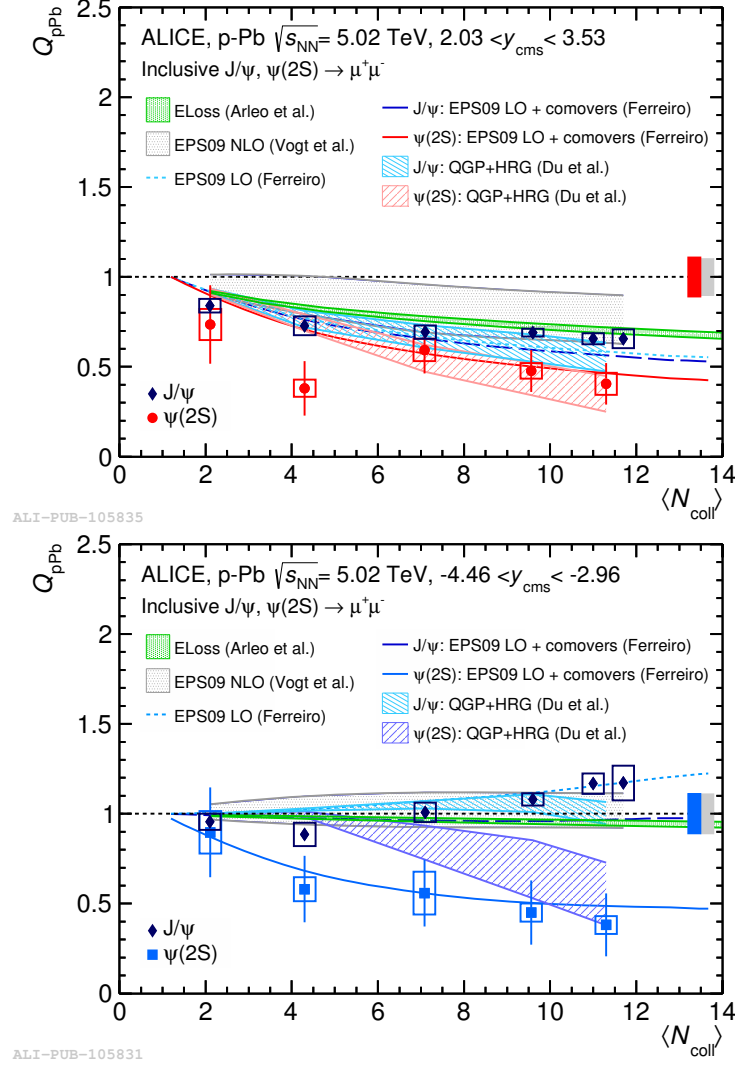
Figure 1.22: J/\psi and \psi(2S) R_{pA} at \sqrt{s_{NN}} = 5.02 TeV as a function of N_{coll} at forward (top) and backward (bottom) rapidities compared to models [129, 133, 152, 153]. The boxes around unity correspond to the global \psi(2S) systematic uncertainties at forward (red box) and backward (blue box) rapidities. The grey box is a global systematic uncertainty common to both J/\psi and \psi(2S) [154].
