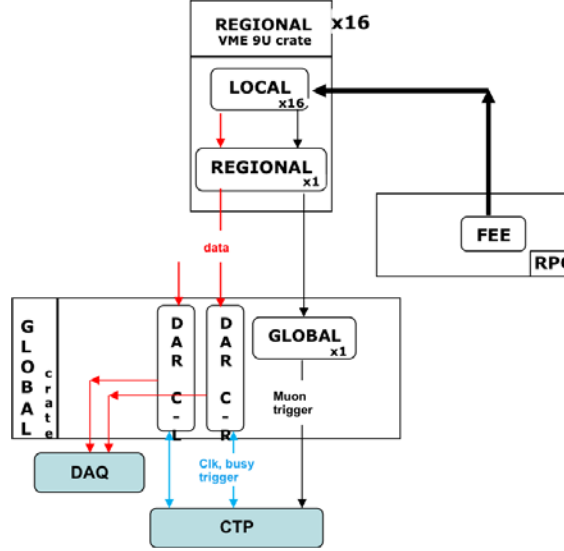
Figure 4.7: Schematic of the MTR readout electronics architecture.
