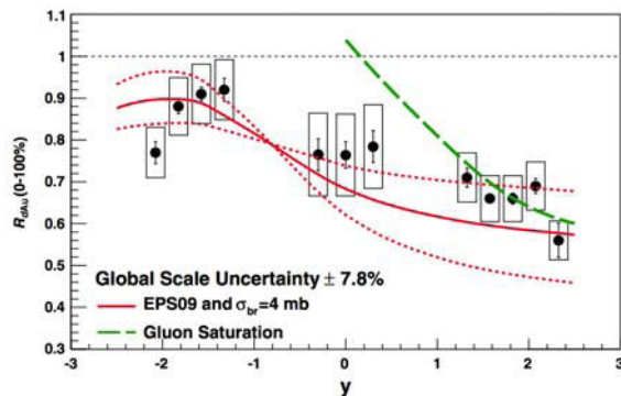
Figure 1.18: J/\psi nuclear modification factor in the centrality range 0-100% as a function of rapidity in d Au collisions measured by PHENIX [144]. Results are compared to EPS09 calculations [113] and calculations incorporating gluon saturation effects [145].
