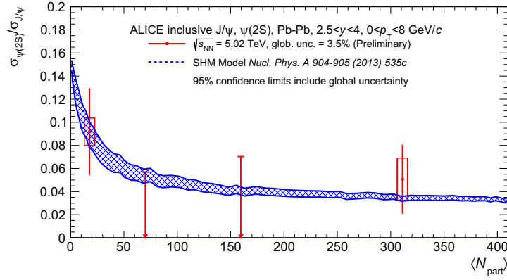
Figure 3.29: \psi(2S) -to- J/\psi ratio versus N_{part} compared to the Statistical Hadronization Model. For the centrality bins where the signal could not be extracted, only the 95% CL is shown. The red box around unity corresponds to the global uncertainty which are included in the confidence limits calculation and therefore do not apply to the CL. Uncertainties in the model correspond to different values of the nucleus density below which nucleons are considered as part of the corona: \rho < 0.1\rho_0 in the upper limit and for \rho < 0.15\rho_0 in the lower limit.
