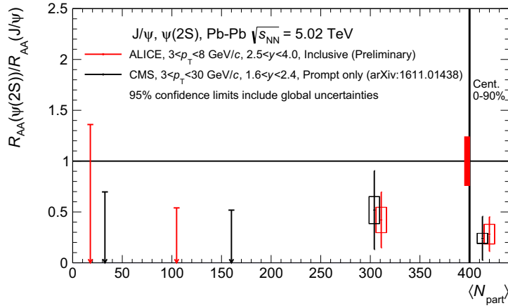
Figure 3.25: Double-ratio R_{AA}^{\psi(2S)}/R_{AA}^{J/\psi} as a function of N_{\text{part}} (red) compared to the values of CMS (black) for p_T > 3 GeV/c. For the centrality bins where the signal could not be extracted, only the 95% confidence limit is shown. The global systematic uncertainty is drawn in the box around unity. The global uncertainties are already included in the confidence limit calculation. The value quoted for N_{\text{part}} > 400 corresponds to the centrality-integrated value (0-90%).
