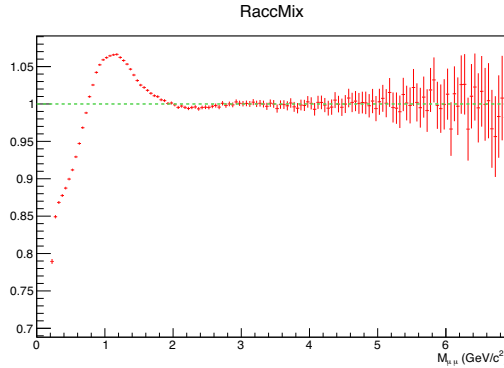
Figure 3.5: Normalization factor R as a function of the invariant mass obtained from events in the 0-10% centrality range.
