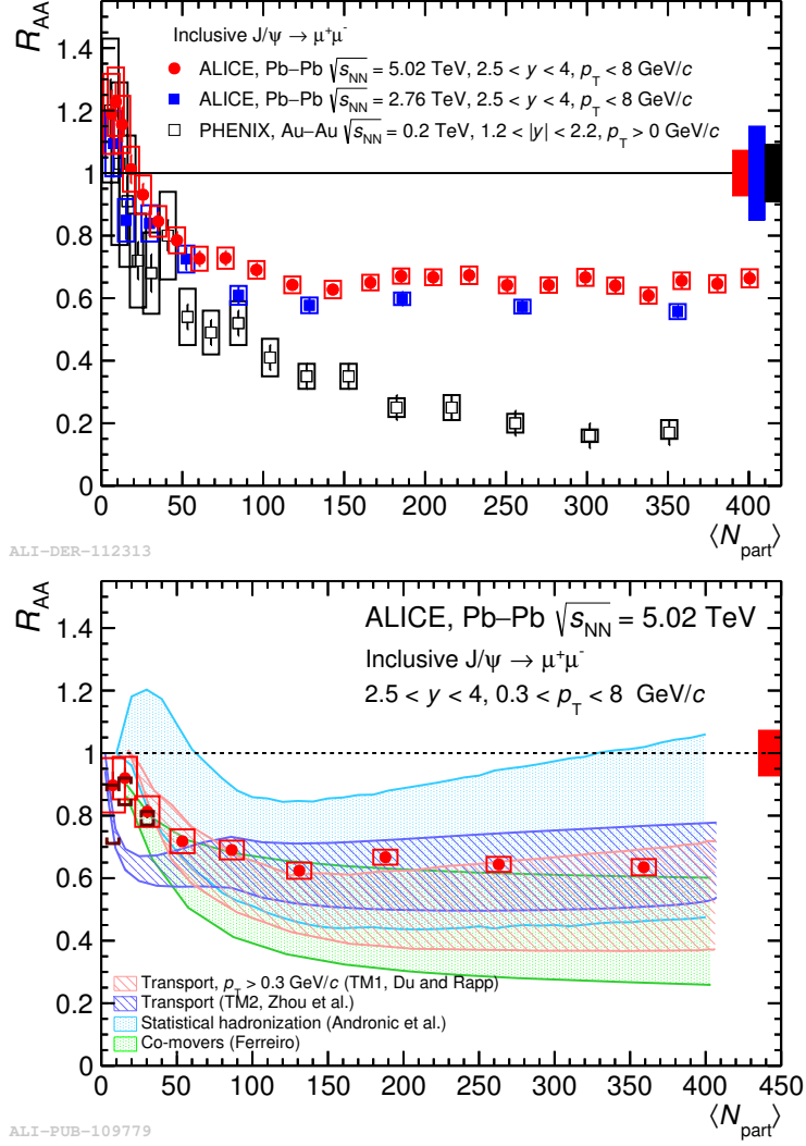
Figure 1.25: Top: Inclusive J/\psi R_{AA} as of function of N_{part} measured in Pb – Pb collisions at \sqrt{s_{NN}} = 2.76 TeV and \sqrt{s_{NN}} = 5.02 TeV compared to PHENIX measurement in Au – Au collisions at \sqrt{s_{NN}} = 0.2 TeV [156, 157]. Bottom: Inclusive J/\psi R_{AA} as of function of N_{part} with a cut p_T > 0.3 GeV measured in Pb – Pb collisions at \sqrt{s_{NN}} = 5.02 TeV compared to models [157].
