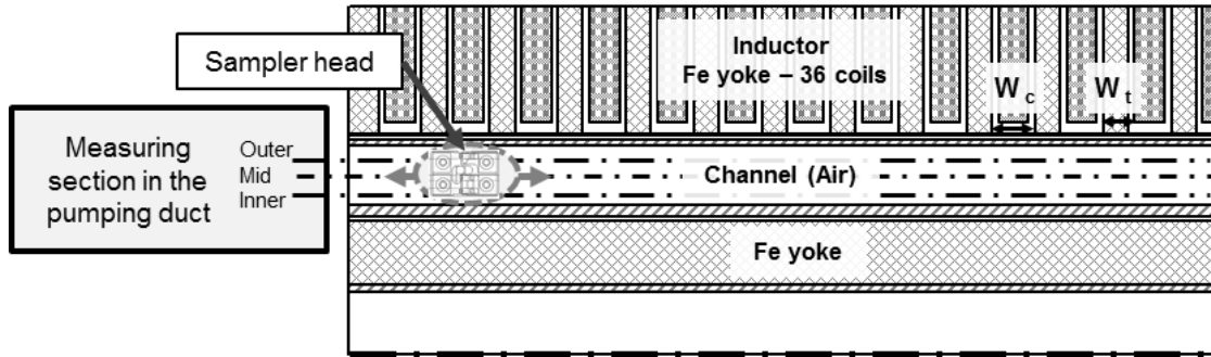
Figure 2: Location of the magnetic field sampler head.
