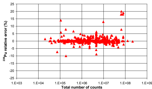
Fig. 2. Relative errors between the ^{239}\text{Pu} mass ratio obtained by IGA and the ^{239}\text{Pu} mass ratio of reference for the global Pu spectrum database according to total number of counts in the spectrum.
