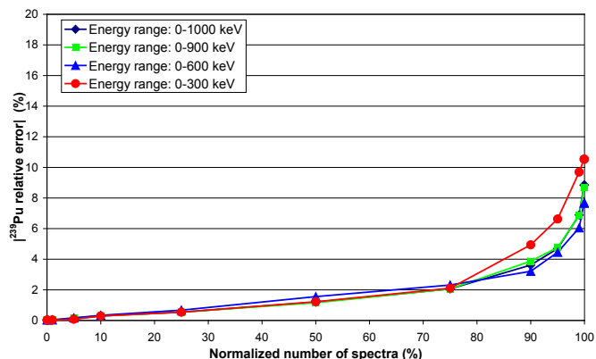
Fig. 4. Relative errors between the ^{239}\text{Pu} mass ratio obtained by IGA and the ^{239}\text{Pu} mass ratio of reference calculated for the original set of spectra with an energy range equal to 0-1 MeV and for the three sets of artificial spectra corresponding to 0-900 keV, 0-600 keV, and 0-300 keV.
