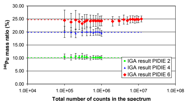
Fig. 9. IGA results for 240 Pu (mean of mass ratios obtained by IGA on ten or more spectra) for the three samples according to the total number of counts in the spectrum. Reference values are displayed with the dotted lines. Error bars correspond to the mean of the uncertainties provided by the code, calculated for the ten spectra of each experimental configuration.
