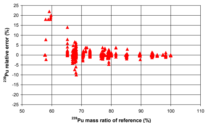
Fig. 3. Relative errors between the ^{239}\text{Pu} mass ratio obtained by IGA and the ^{239}\text{Pu} mass ratio of reference for the global Pu spectrum database according to ^{239}\text{Pu} mass ratio.
