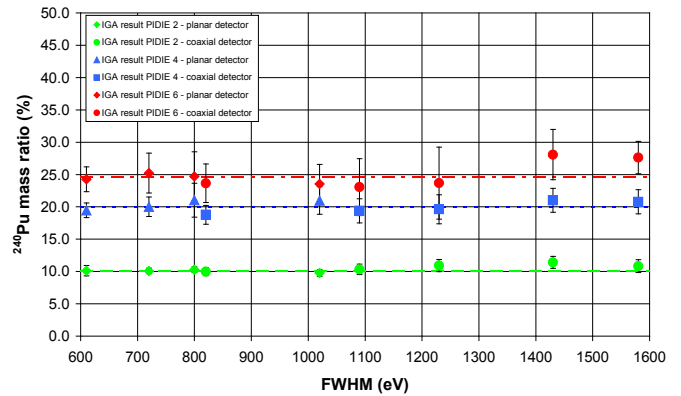
Fig. 11. IGA results for ^{240}\text{Pu} (mean of mass ratios obtained by IGA on ten or more spectra) for the three samples according to FWHM measured at 122 keV (counting statistics: 10^6 counts, gain 0.075 keV/channel). Reference values are displayed with the dotted lines. Error bars correspond to the mean of the uncertainties provided by the code, calculated for the ten spectra of each experimental configuration.
