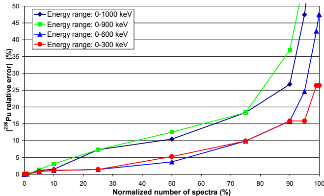
Fig. 7. Relative errors between the ^{238}\text{Pu} mass ratio obtained by IGA and the ^{238}\text{Pu} mass ratio of reference calculated for the original set of spectra with an energy range equal to 0-1 MeV and the three sets of artificial spectra corresponding to 0-900 keV, 0-600 keV, and 0-300 keV.
