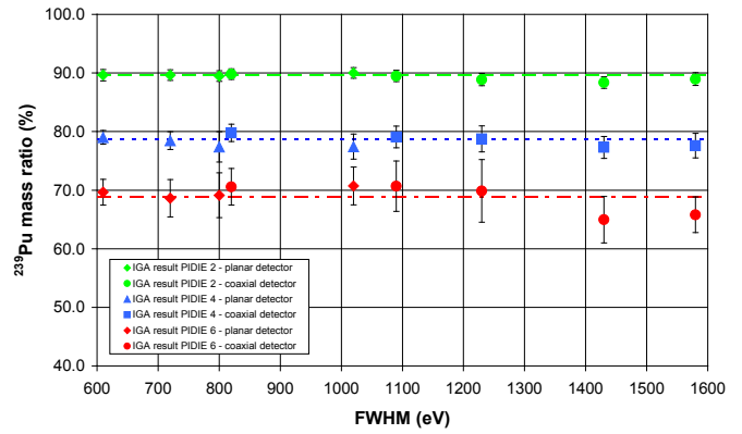
Fig. 10. IGA results for ^{239}\text{Pu} (mean of mass ratios obtained by IGA on ten or more spectra) for the three samples according to FWHM measured at 122 keV (counting statistics: 10^6 counts, gain 0.075 keV/channel). Reference values are displayed with the dotted lines. Error bars correspond to the mean of the uncertainties provided by the code, calculated for the ten spectra of each experimental configuration.
