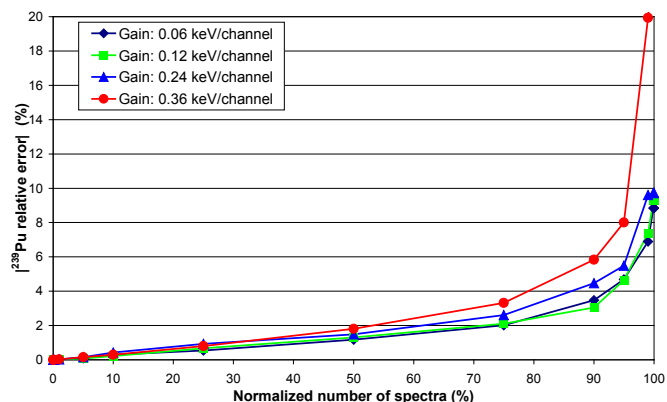
Fig. 5. Relative errors between the ^{239}\text{Pu} mass ratio obtained by IGA and the ^{239}\text{Pu} mass ratio of reference calculated for the original set of spectra with a gain equal to 0.060 keV/channel and for the three sets of artificial spectra corresponding to 0.120 keV/channel, 0.240 keV/channel, and 0.360 keV/channel.
