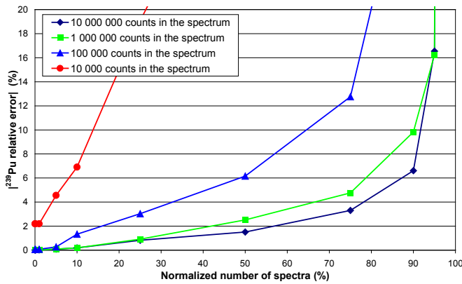
Fig. 6. Relative errors between the ^{239}\text{Pu} mass ratio obtained by IGA and the ^{239}\text{Pu} mass ratio of reference calculated for the original set of spectra with a counting statistics equal to about 10^7 counts and for the three sets of artificial spectra corresponding to 10^6 counts, 10^5 counts, and 10^4 counts in the spectrum.
