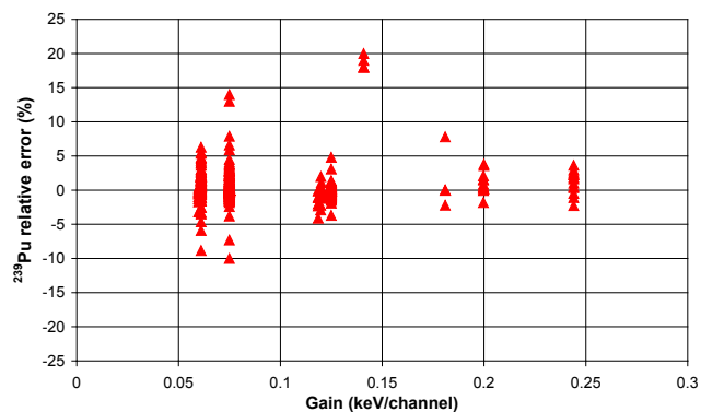
Fig. 1. Relative errors between the ^{239}\text{Pu} mass ratio obtained by IGA and the ^{239}\text{Pu} mass ratio of reference for the global Pu spectrum database according to gain.
