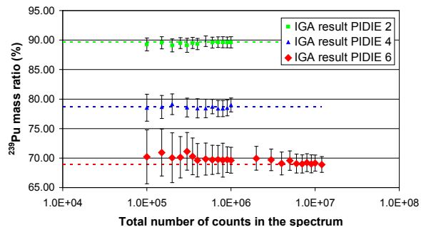
Fig. 8. IGA results for 239 Pu (mean of mass ratios obtained by IGA on ten or more spectra) for the three samples according to the total number of counts in the spectrum. Reference values are displayed with the dotted lines. Error bars correspond to the mean of the uncertainties provided by the code, calculated for the ten spectra of each experimental configuration.
