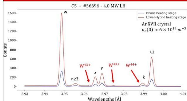
Fig. 9: Spectra from Ar XVII crystal w/o line-doubling
