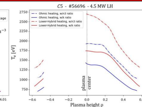
Fig. 10: Te LOS-profiles, for Ohmic and Lower Hybrid heating stages, from the resonance line w to the dielectronic satellite k line ratio and to n \geq 3 satellites line ratio
