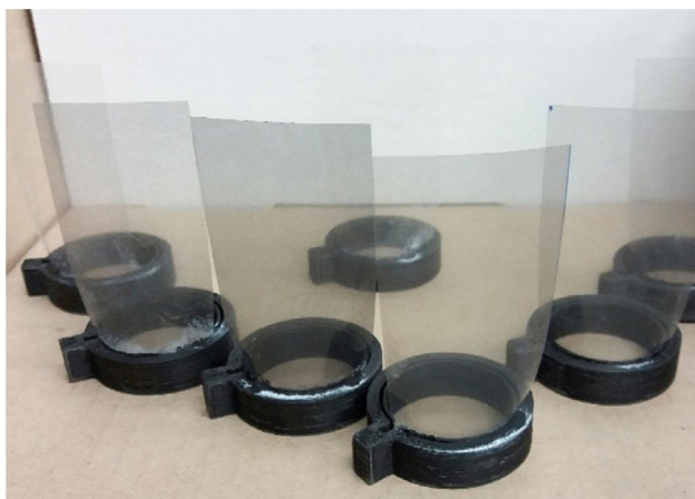
Fig. 9. Filters with different neutral density. The filters shown here were designed to cover only one PMT.
