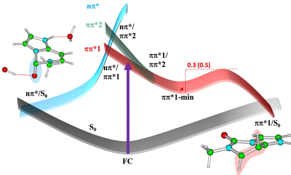
Figure 3. Schematic description of the proposed decay mechanism for \epsilon\text{C} and \epsilon\text{CH}^+ in water. The value in parentheses is relative to \epsilon\text{CH}^+ . Schematic drawing of a representative structure of the \pi\pi^*1/S_0 and n\pi^*/S_0 crossing regions are also shown for \epsilon\text{CH}^+ and \epsilon\text{CH}^+\cdot 2\text{H}_2\text{O} .
