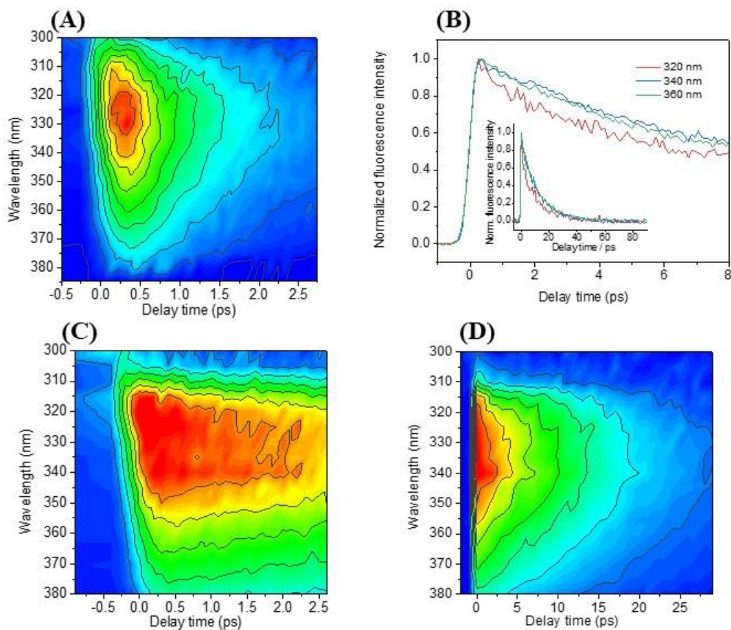
Figure 2. Corrected time-resolved fluorescence spectra after laser excitation at \lambda_{exc}= 267 nm of \epsilon dC in PBS at pH 7.4 (A), \epsilon dCH^+ in citrate buffer at pH 3 over a time window of 3 ps (C) and 30 ps (D)*. Fluorescence decays obtained for a solution of \epsilon dCH^+ in citric acid at different emission
