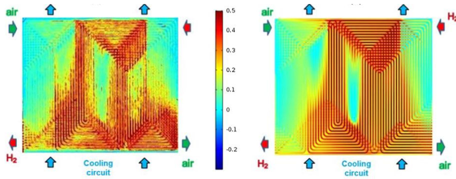
Figure 2. Comparison between measured (left) and simulated (right) total water thickness at 0.25\text{A}/\text{cm}^2 and 64^\circ\text{C} at cell scale [3].
