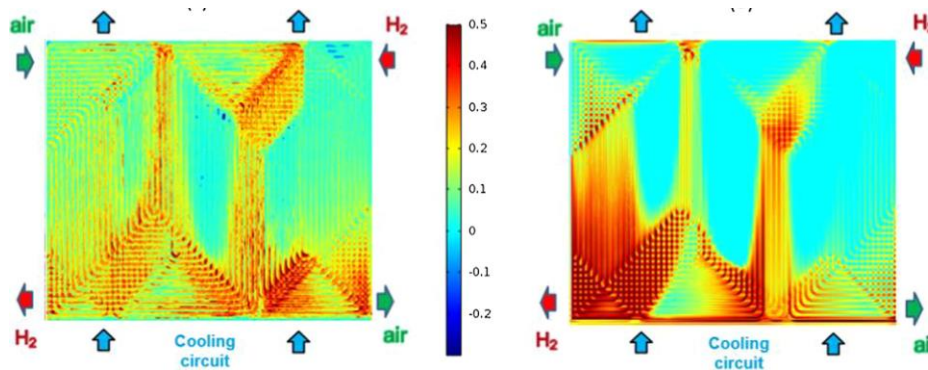
Figure 3. Comparison between measured (left) and simulated (right) total water thickness at 1\text{A}/\text{cm}^2 and 59^\circ\text{C} at cell scale [3].
