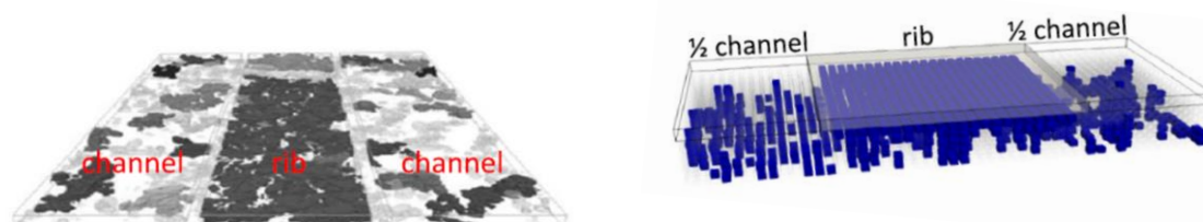
Figure 1. Comparison between experimental measurement [5] of water distribution by X-ray tomography (left) and simulated result (right) [1] at same operating conditions (80°C, 0.75A/cm 2 , 100%RH in channel)
