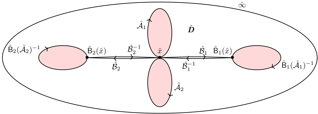
FIGURE 4. The external boundary should be thought of as the point \hat{\infty} . The domain \hat{D} \subset \hat{C} is the complement of the coloured regions.
