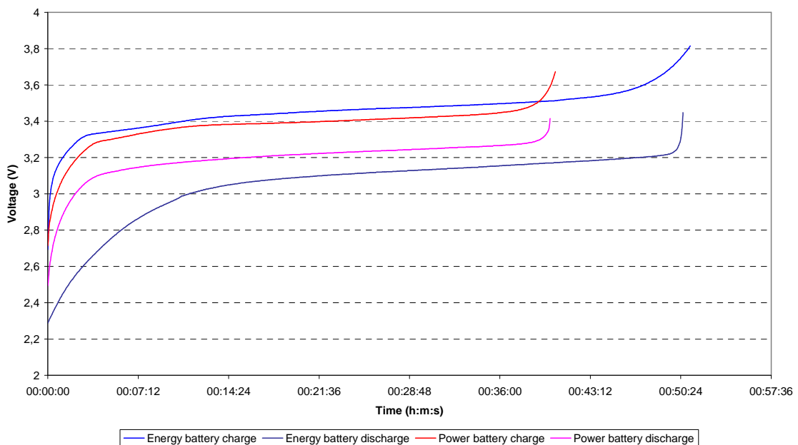
Figure 6 : Voltage hysteresis comparison
