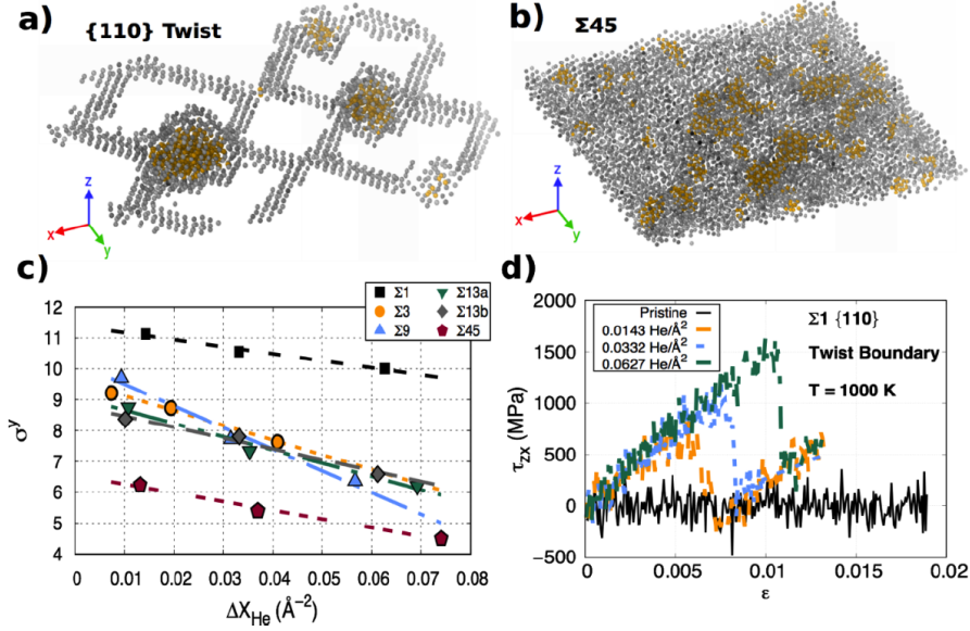
Figure 18: He segregation to a) {110} twist and b) \Sigma 45 interfaces. W and He atoms are shown in gray and orange, respectively. c) Yield stress upon normal loading depending on interface misorientation and He content. d) Stress-strain response of the system containing a {110} twist interface upon shear depending on He content. Images courtesy of E. Martinez, Los Alamos National Laboratory.
