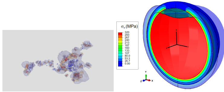
Figure 17: Left: stress isosurfaces induced by a typical 150 keV cascade in tungsten[31]. Vacancies (blue spheres) and interstitials (red spheres) are identified by a Wigner-Seitz cell analysis and isosurfaces of stress are indicated (yellow- trace of dipole tensor = +0.1eV, blue- trace of dipole tensor = -0.01eV). Right: Radial stress computed using the finite element method for a spherical model reactor pressure vessel with the cap of the sphere shielded[206]. These two calculations are linked together by the simple formula, equation (7), relating internal body forces to the density of relaxation volumes of defects in the microstructure of irradiated material. Figure reproduced from Ref. [206].
