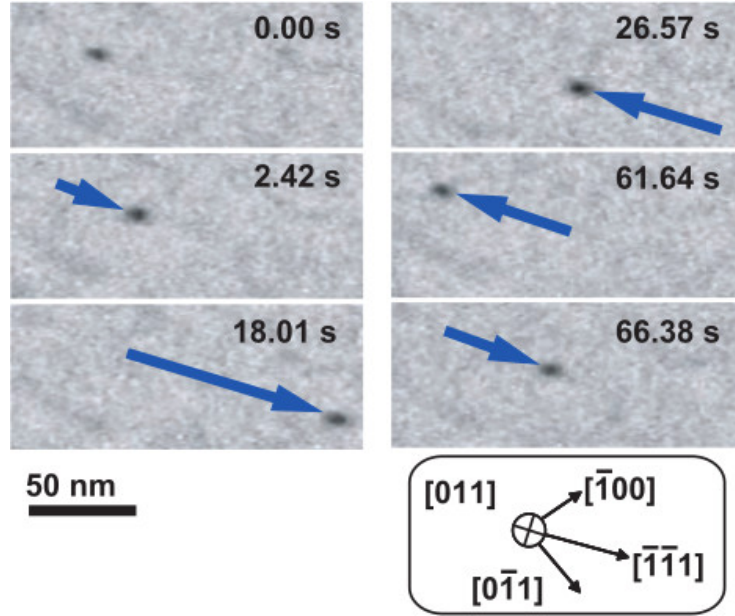
Figure 9: One dimensional diffusion of a \frac{1}{2}[11\bar{1}] loop in ultra-high purity Fe at 575 K observed using in-situ TEM. From Ref. [96], reprinted with permission from AAAS.
