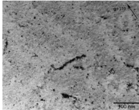
Figure 8: Example of TEM characterization of damage produced by 500 keV Fe^+ irradiation of a UHP Fe thin film at room temperature and 0.5 dpa. From Ref. [95], reprinted with permission from Elsevier.
