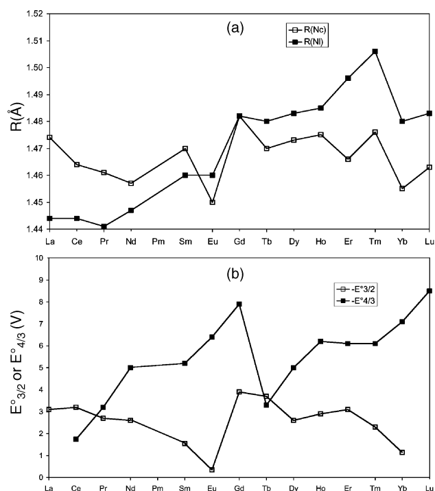
Fig. 1 (a) Lateral and central nitrogen radii in the crystal compounds [\text{Ln}(\text{tpy})\text{Cl}(\text{H}_2\text{O})_y]^{3+} along the Ln series. (b) Experimental and calculated E^{\circ}_{3/2} and E^{\circ}_{4/3} redox potentials along the Ln series. 14
