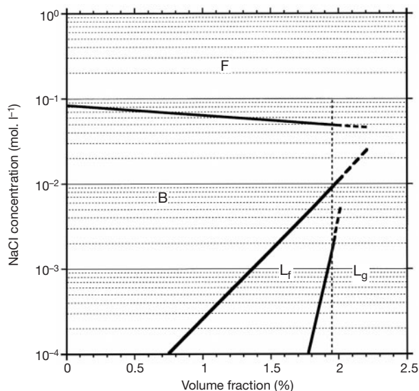
Figure 3 Phase diagram of H_2Sb_3P_2O_{14} suspensions versus volume fraction and salt concentration. Upon decreasing the volume fraction, the suspensions first form a lamellar gel phase ( L_g ), then a lamellar fluid phase ( L_f ) and finally enter a biphasic regime (B). The system flocculates (F) at high salt molarity.
