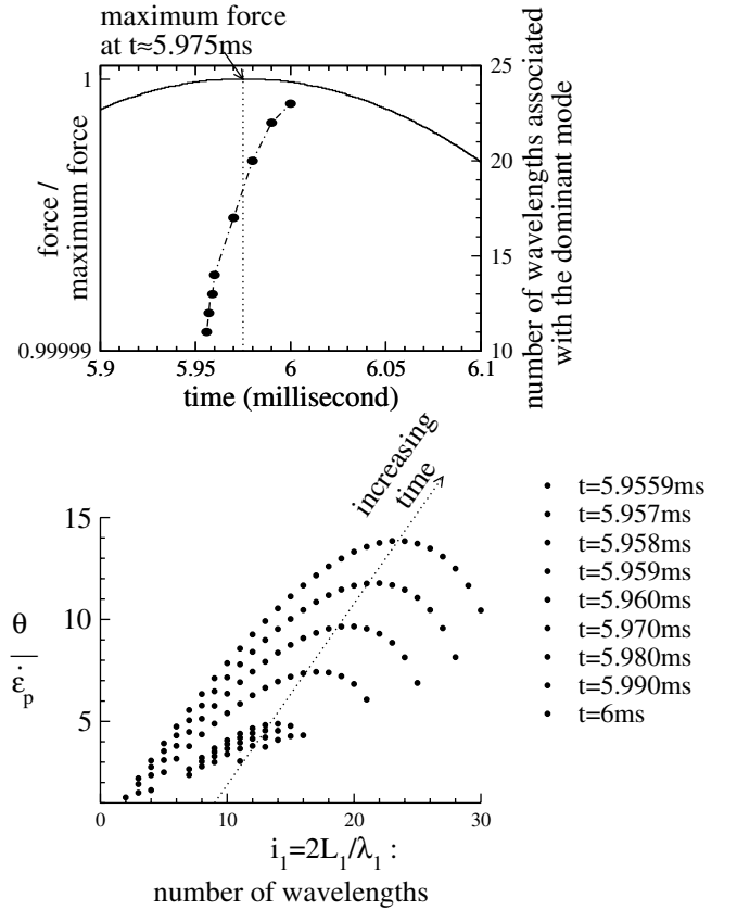
Fig. 9. Plane strain tension on a non viscous material. Initial thickness: 2L_{03} = 2 cm – initial velocity gradient: V_{01}/L_{01} = 10 s -1 with L_{01} = 10 m – material: idem Figure 8, except \varepsilon_i = 0.1 .
