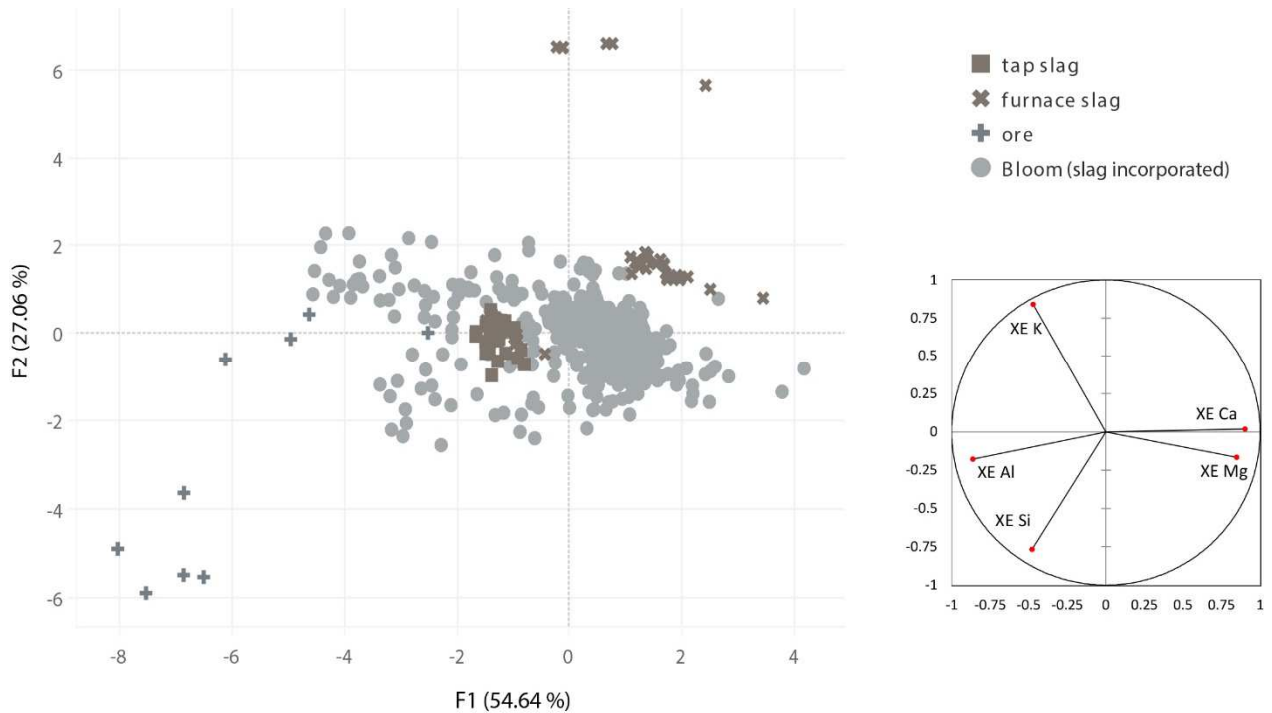
Figure 12: Multivariate plot of the sub-composition values of the non-reduced compounds (NRC ratios XE) from major elemental analyses in ore, furnace slag, tap slag and slag incorporated to the bloom. The comparison is done using the element composition.
