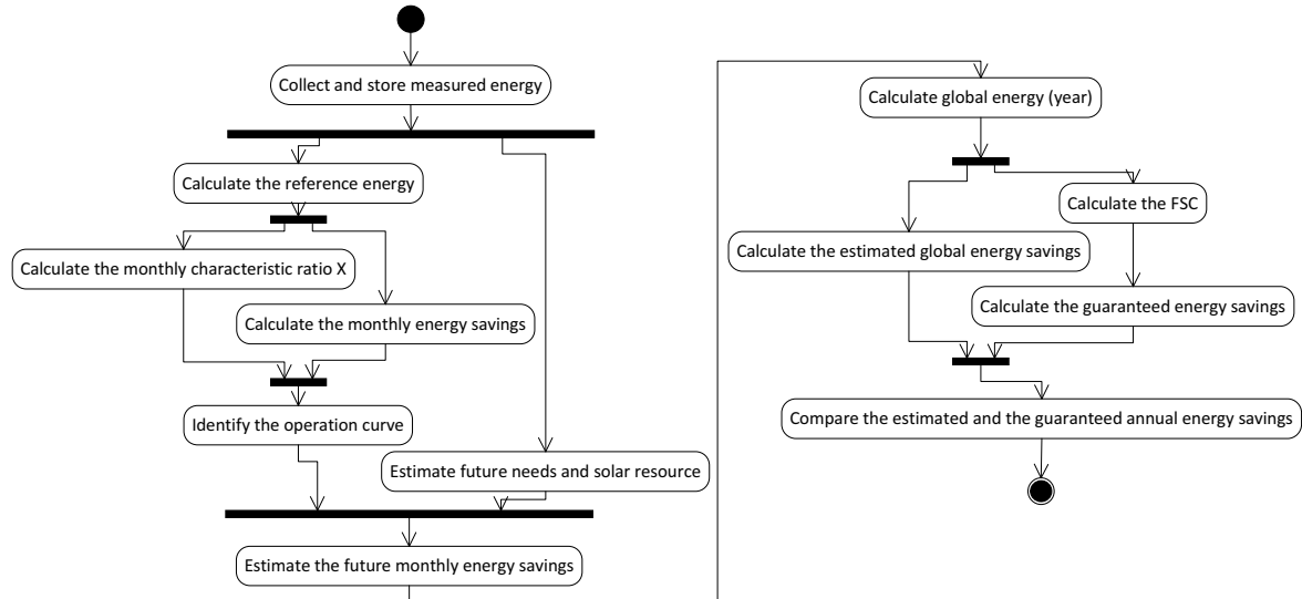
Fig. 3: Global diagram of the operations to be done monthly for the proposed monitoring procedure
