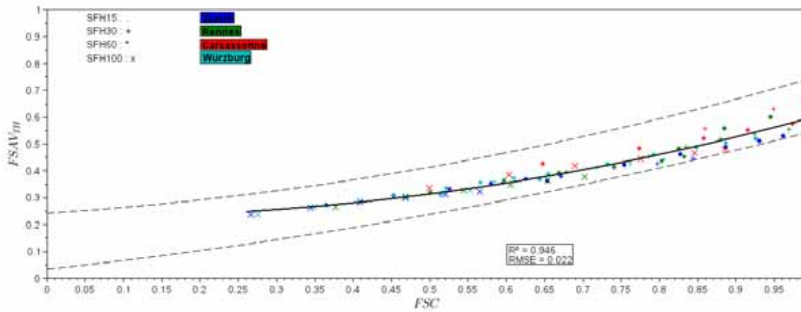
Fig. 2: FSAV-FSC curve of the studied SCS
