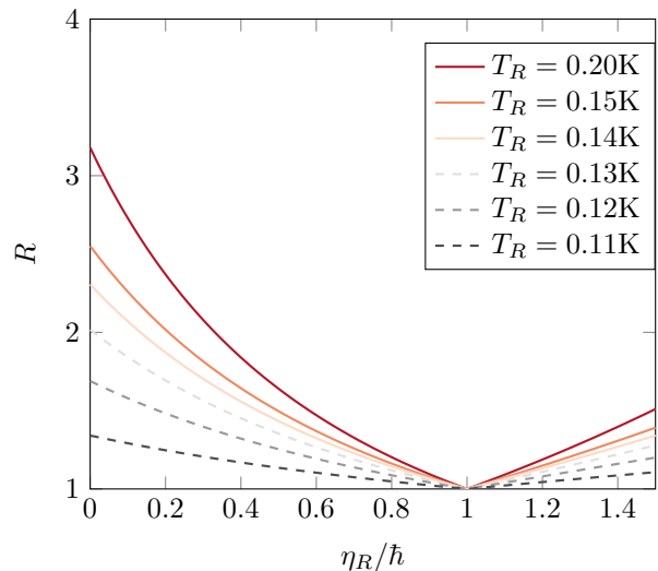
FIG. 4: Rectification index R , as defined in (60), for different values of T_R and T_L = 0.1\text{K} . The other parameters are given in the caption of figure 3
