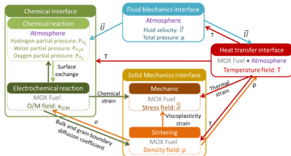
Figure 6 : Multi-physics modelling of the sintering step
