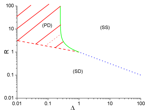
FIG. 1. "Pseudo phase diagram" resulting from the irradiation of non-miscible alloys as a function of the reduced units \Delta and R irrespective of their overall composition. Three distinct domains can be produced : a disordered domain associated with a solid solution (SS), a domain where the spinodal decomposition (SD) takes place and a pattern domain (PD) where the coarsening of precipitates is frozen. (dashed red line: limit between the spinodal decomposition and patterning of domains ( \Delta_{min} ), blue dotted line: limit between the (PD) and the (SS))
