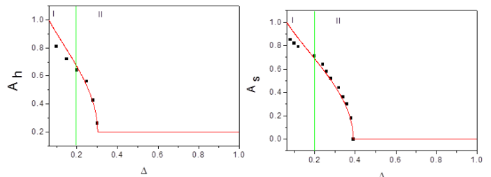
FIG. 4. Comparison of solubility limits A_s and A_h (full red line) calculated from the minimization of the 2D SH functional and extracted from 2D numerical simulations (black squares) for the honeycomb (left, \bar{\psi} = 0.25 ) and the labyrinthine (right, \bar{\psi} = 0 ) micro-structures for different \Delta values ( R = 3 ).
