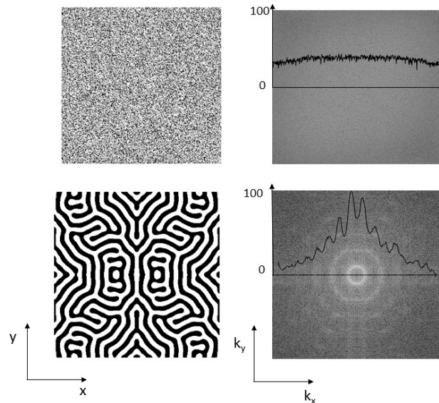
FIG. 2. 2D simulation of a random distribution of a Ag_{0.38}Cu_{0.62} alloy, before (top ) and after (bottom ) irradiation with 1 MeV Kr ions at \phi = 6 \times 10^{12} cm^{-2} s^{-1} , and T = 440K obtained from the numerical solution of Eq.( 3) ( R = 3 and \Delta = 0.2 ). Initial (up left-hand side) and final (down left-hand side) 2D micro-structures in real space and their corresponding Power Spectral Density (PSD) in the Fourier space (right-hand side) are plotted. In these simulations, A rich (black) (B rich (white)) domains are associated with positive (negative) \eta values (the 2D domain size is equal to 200 in reduced units). At late-time, the PSD is radially symmetric and peaks sharply around k_0 (intense white ring). Late-time structure factors S(k, t) , resulting from a circular average of the PSD for both initial (top) and final micro-structures (bottom), are plotted as a full line along the k_x component of the wave vector.
