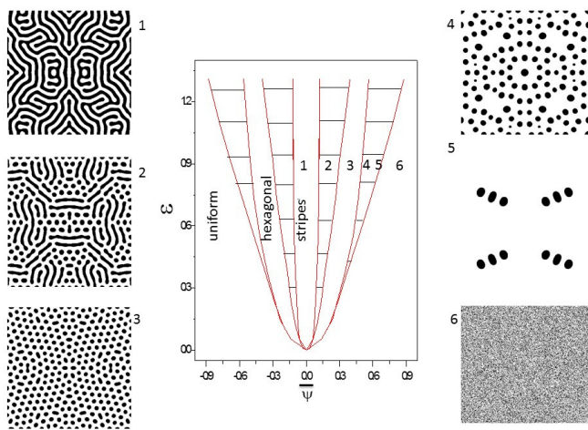
FIG. 3. Proposed generic 2D "Pseudo phase diagram" in the (PD) area derived from the SH functional as function of the nominal composition, \bar{\psi} and the \epsilon(R, \Delta) parameter. The solid lines represent the limits between different micro-structures and the hatched area is associated with coexistent domains. This "pseudo phase diagram" is in fair agreement with 2D simulated microstructures (graphs 1 to 6) resulting from the numerical resolution of Eq. (3) (From top-left to bottom-right, 1: \bar{\psi} = 0 , 2: \bar{\psi} = 0.2 , 3: \bar{\psi} = 0.35 , 4: \bar{\psi} = 0.5 , 5: \bar{\psi} = 0.65 , 6: \bar{\psi} = 0.7 and \epsilon = 0.85 ).
