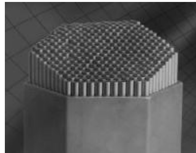
Fig. 1. Picture of a fuel sub-assembly, with a hexagonal tube wrapping the fuel pins (Ref. 1).
