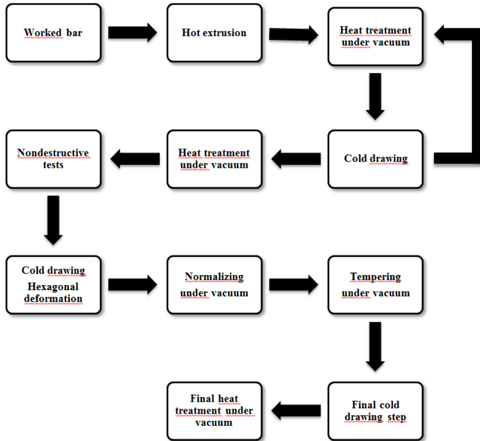
Fig. 2. Manufacturing process used for the hexagonal tubes of Phénix sub-assemblies.
