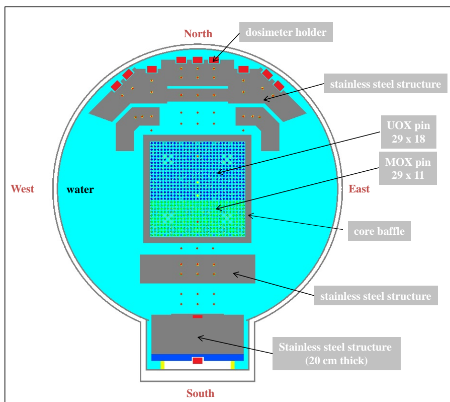
Figure 1: FLUOLE-2 device
