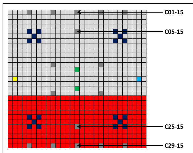
Figure 5: fission chamber loading
