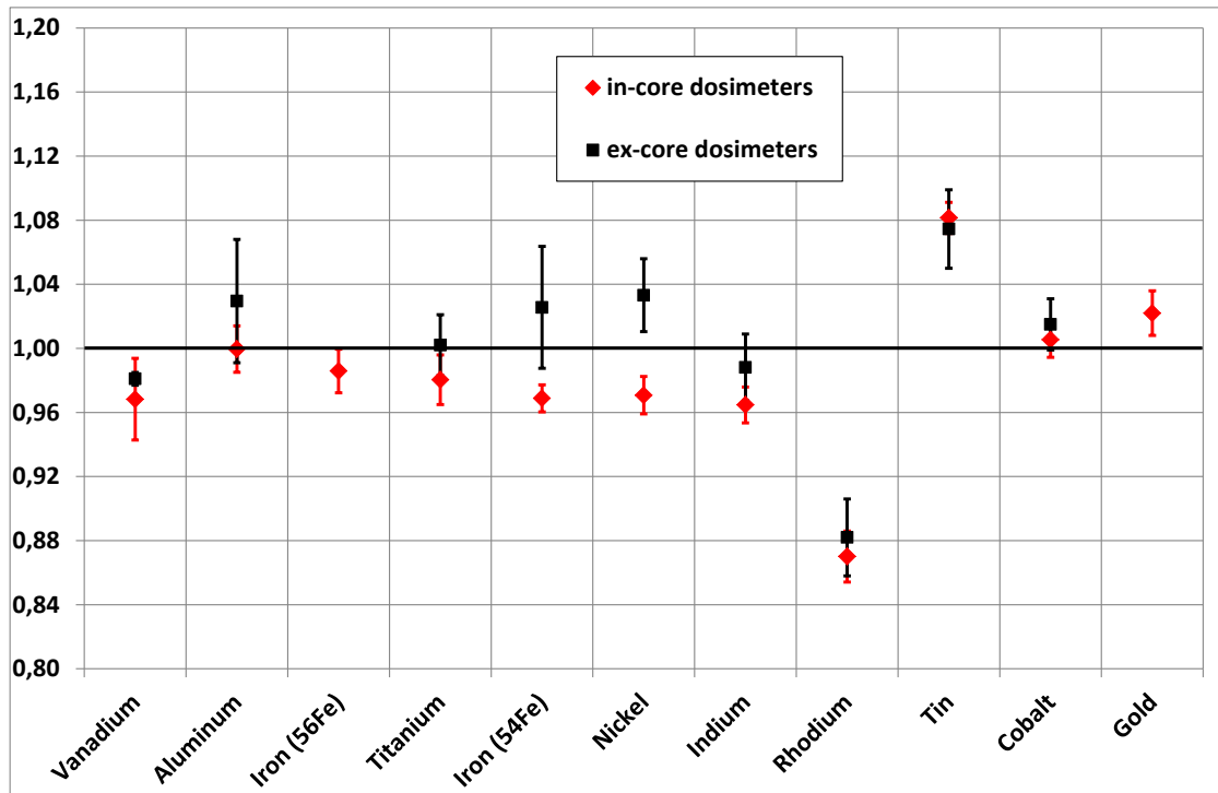
Figure 4: dosimeter analysis: synthesis
