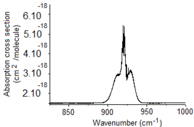
Fig. 4. Approximate absorption cross section for \text{RuO}_4 in the 10^{-12}\text{ }\mu\text{m} atmospheric window. Approximately 10 mbar of ruthenium tetroxyde in 1012mbar nitrogen at 298K.
