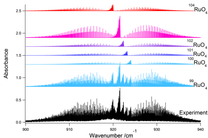
Fig. 1. Overview of the \nu_3 region of natural abundance \text{RuO}_4 , compared to the simulation. The five upper curves are simulations for individual isotopologues.
