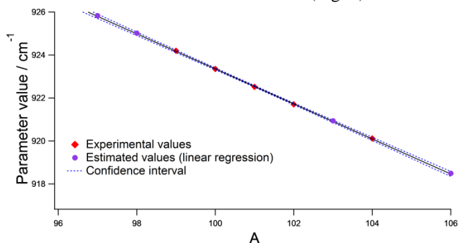
Fig. 2. Estimate of the \nu_3 band center parameter for minor isotopologues through linear regression.
