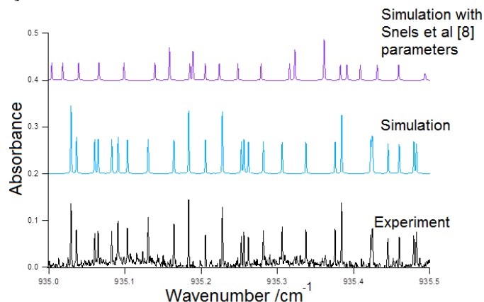
Fig. 3. Comparison between this work and precedent work of simulation for high J values ( 65 < J < 68 ).
