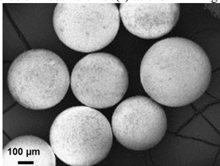
Fig. 2. FEG-SEM micrograph in electron secondary mode of cerium oxide microspheres obtained from the WAR process and calcined at 800°C in air.
