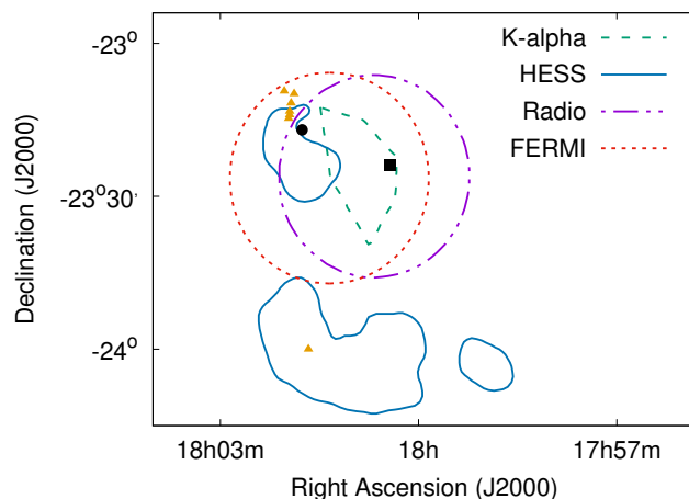
Fig. 1. Contour map for the W28 region. The approximate radio boundary of the SNR shell is shown as a purple dot-dot-dashed circle. The solid blue contours represent the 4\sigma significance excess TeV emission observed by H.E.S.S. (Aharonian et al. 2008). The short-dashed red circle is the best-fit disk size for the Fermi -LAT GeV source associated to the northeastern MC (Cui et al. 2018). The enhanced region of Fe I K\alpha line emission is the area enclosed by the dashed green line (Nobukawa et al. 2018). The CR ionization rate has been measured from IRAM observations pointed in the directions indicated by the yellow triangles (Vaupré et al. 2014). The filled black circle and square indicate the centroids of the X-ray emission for the northeast and central X-ray sources, respectively (Rho & Borkowski 2002).
