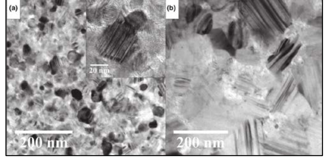
Fig. 2. TEM images of the as-received (a) HNS and (b) TSA3 fibers. Stripped patterns inside the grains indicate the high density of stacking faults in both samples. Reproduced from Ref. 5
