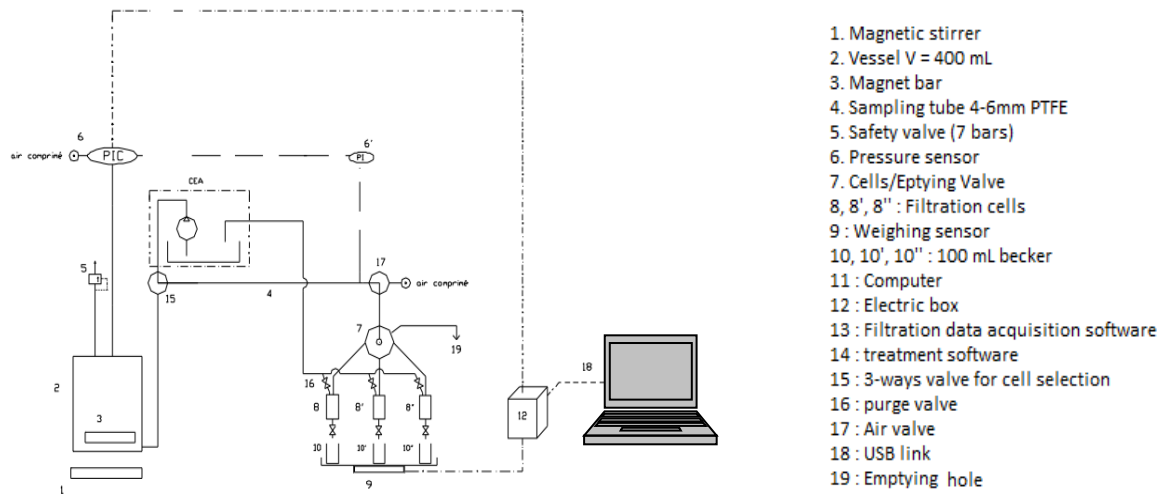
Figure 1 : Minitest of filterability
