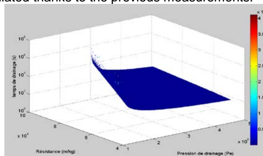
Figure 2 : Deliquoring time for a target of 22% of humidity for cubic shape of calcium carbonate
