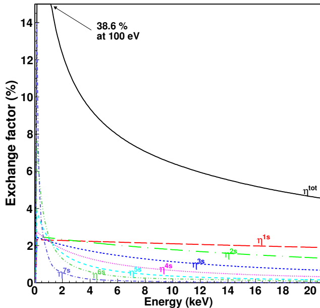
FIG. 1. (Color online) Total exchange factor for the ^{241}\text{Pu} beta decay and contributions of each orbital. The effective nuclear charges used are the relativistic ones from Harston and Pyper [7] (see Table II).
