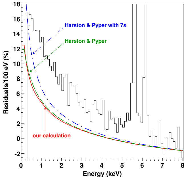
FIG. 3. (Color online) Residuals relative to the allowed spectrum for the measured spectrum of ^{241}\text{Pu} from Loidl et al. [1], for our calculation including the exchange effect (red solid line), for the one from Harston and Pyper [7] (green long-dashed line), and for the latter one including the 7s orbital (blue chain-dashed line). The details of the calculations are explained in the text.
