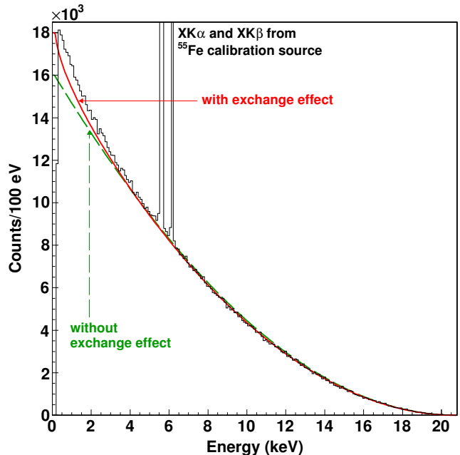
FIG. 2. (Color online) Comparison between the measured beta spectrum of ^{241}\text{Pu} from Loidl et al. [1] and an allowed spectrum calculated with and without exchange effect. The effective nuclear charges used are the relativistic ones calculated for a neutral Pu atom (see Table II).
