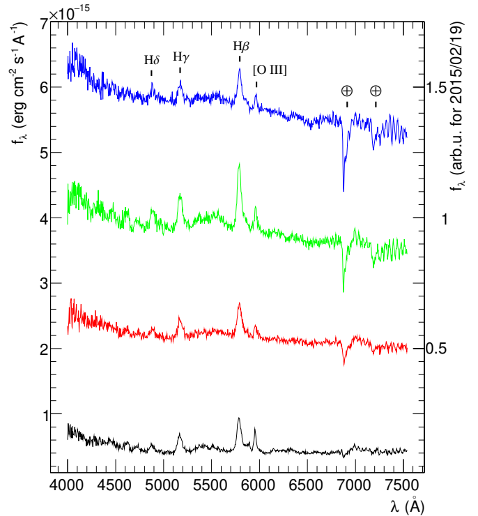
Fig. 3. Optical spectra (4000–7500 Å) of PKS 0736+017 obtained with SPOL on three consecutive nights in 2015: February 18 (in red), February 19 (in green), and February 20 (in blue). Due to the absence of photometric conditions on February 19, this spectrum is provided in arbitrary units. For reference, shown in black is a spectrum from a low state of the source (February 9, 2016). The emission lines and telluric features are identified in the spectrum from February 20, 2015.
