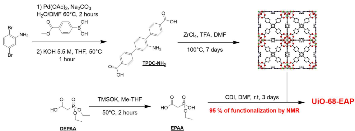
Figure 1 : Schematic synthesis pathway for UiO-68-EAP
