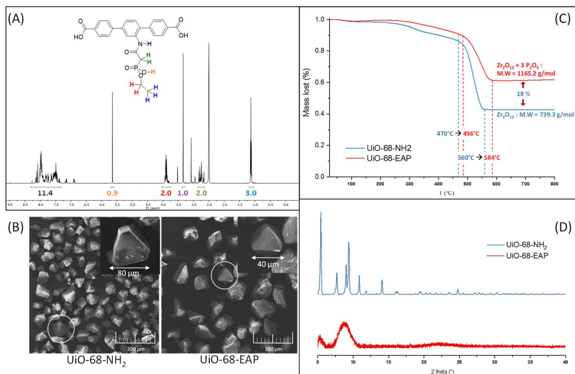
Figure 2: ^1\text{H} NMR analysis of the digested UiO-68-EAP (A); Characterization of UiO-68-EAP and UiO-68-NH 2 by SEM (B), TGA (C), and PXRD (D)
