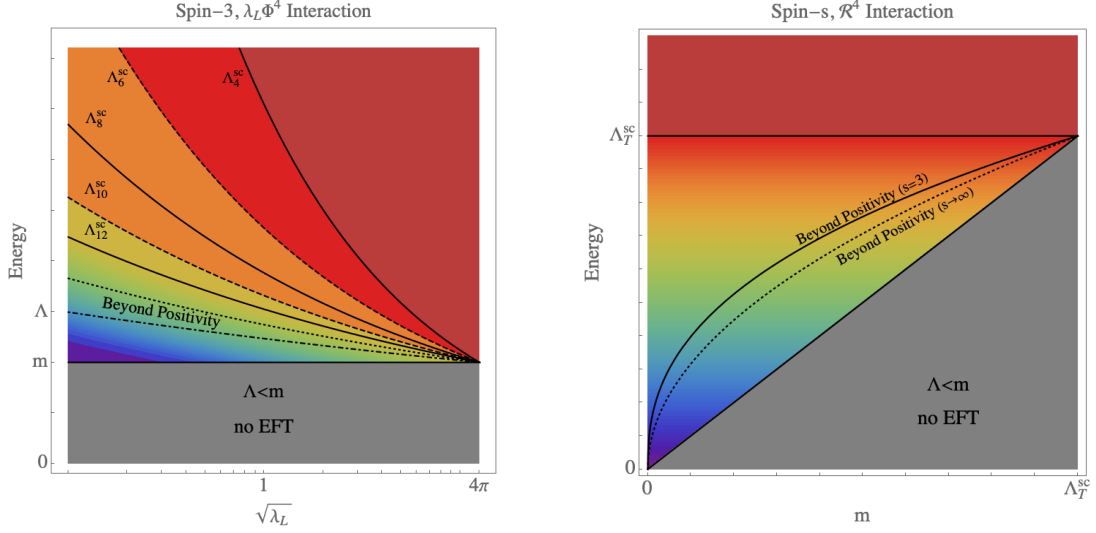
Figure 1: LEFT : Different strong-coupling scales for s = 3 as function of \sqrt{\lambda_L} in Eq. (1.31) or Eq. (2.29). For E \gtrsim m the interaction strength increases at high energy; the S(V) polarizations are strongly coupled at \Lambda_{12}^{\text{sc}}(\Lambda_8^{\text{sc}}) generically (solid lines) or at \Lambda_{10}^{\text{sc}}(\Lambda_6^{\text{sc}}) for the tuned theory (dashed lines). Beyond-positivity bounds for the \lambda_L \Phi^4 interaction (dotted) and \lambda_L \partial^4 \Phi^4 / \Lambda^4 (dot-dashed): this represents the maximal cutoff \Lambda of the theory, well below the strong-coupling scales. RIGHT : similar energy scales and beyond-positivity bounds for the \mathcal{R}^4 interaction as function of m (solid line for s=3 , dotted for s \rightarrow \infty ).
