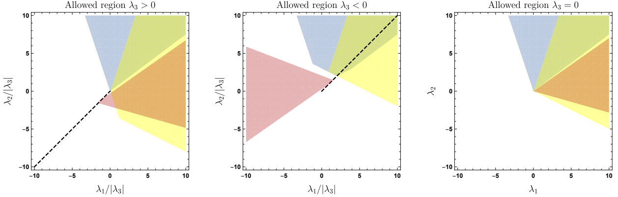
Figure 2: Allowed regions of the coefficients \lambda_1, \lambda_2 as function of the sign of \lambda_3 . Blue: result from scattering of linear-definite polarizations Eq. (2.28). Red: result from \Sigma_{IR}^{(2)} > 0 by scattering different choices of linear combination of polarizations. Yellow: result from \Sigma_{IR}^{(4)} > 0 by scattering only linear-definite polarizations. The dotted line correspond to the tuning \lambda_1 = \lambda_2 = -\lambda_3 in Eq. (2.8).
