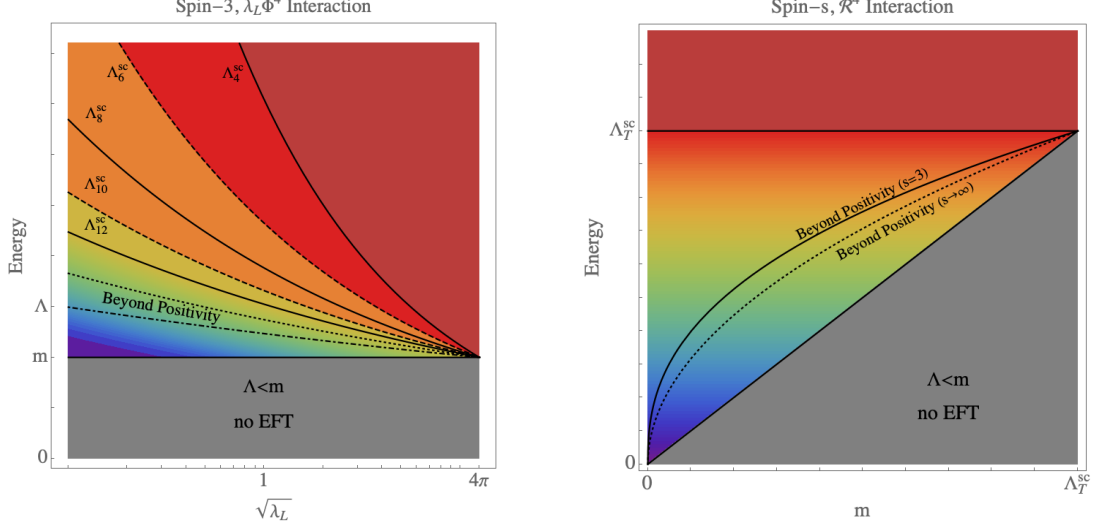
Figure 1: LEFT : Different strong-coupling scales for s = 3 as function of \sqrt{\lambda_L} in Eq. (1.31) or Eq. (2.29). For E \gtrsim m the interaction strength increases at high energy; the S(V) polarizations are strongly coupled at \Lambda_{12}^{\text{sc}}(\Lambda_8^{\text{sc}}) generically (solid lines) or at \Lambda_{10}^{\text{sc}}(\Lambda_6^{\text{sc}}) for the tuned theory (dashed lines). Beyond-positivity bounds for the \lambda_L \Phi^4 interaction (dotted) and \lambda_L \partial^4 \Phi^4 / \Lambda^4 (dot-dashed): this represents the maximal cutoff \Lambda of the theory, well below the strong-coupling scales. RIGHT : similar energy scales and beyond-positivity bounds for the \mathcal{R}^4 interaction as function of m (solid line for s=3 , dotted for s \rightarrow \infty ).
