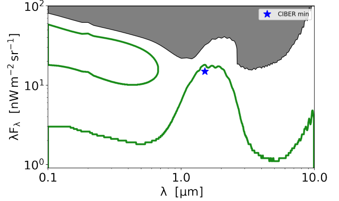
Fig. 4. Cross section of three dimensional parameter space calculated for the bump width \sigma = 0.2 \mu\text{m} . The cross sections of 95% confidence level upper bound and the 68% confidence level contour around the best-fit value for the normalisation of the log-Gaussian EBL bump as a function of the central wavelength are shown with grey and green correspondingly. The data of 1ES 1218+304 are used. Blue star shows the measurement of the minimal EBL bump by CIBER (Matsuura 2017).
