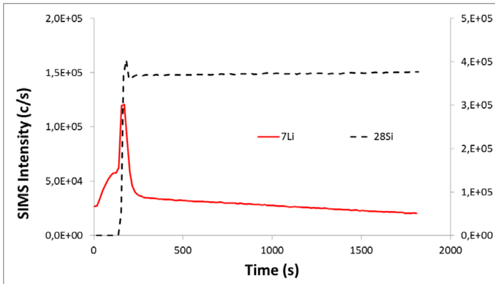
Figure 8: SIMS profiles from the SiC surface in contact with the B 4 C disc. The scale of the dashed curve is on the left side, the scale of the plain curve on the right side.
