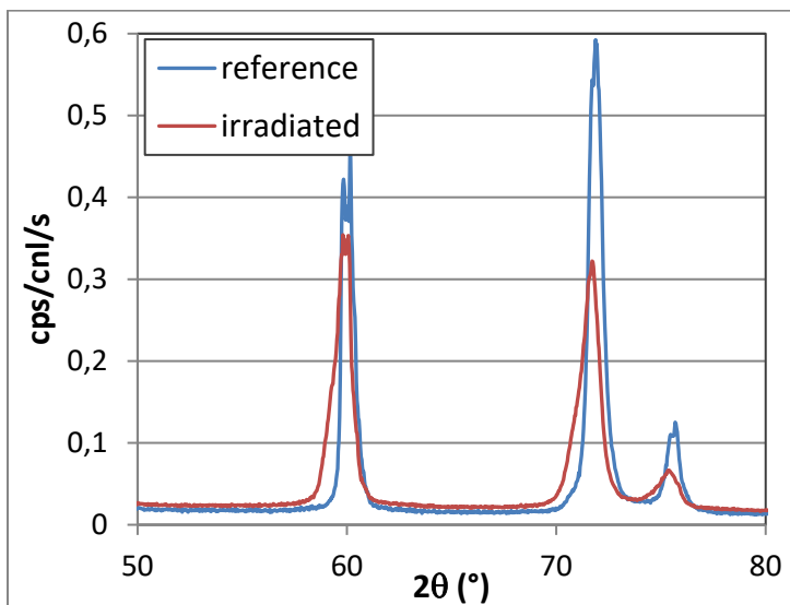
Figure 9. XRD diagrams of the surface of the SiC disc in contact with the B 4 C disc.
