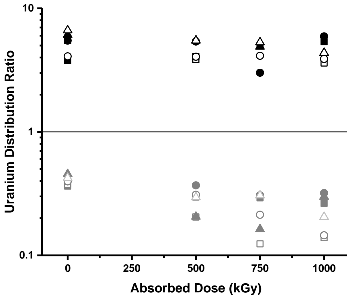
Figure 10: Uranium solvent extraction ( D_U ) from 6.5 M HNO 3 , (black symbols) and stripping (with 0.1M HNO 3 ), (grey symbols) using irradiated, initially 1 M DEHiBA in dodecane. Irradiated organic phase only (solid squares); sparged organic phase (open squares); contact with 0.1 M HNO 3 (solid circles); sparged contact with 0.1 M HNO 3 (open circles); contact with 4 M HNO 3 (solid triangles); and sparged contact with 4 M HNO 3 (open triangles). Mean error bars of \pm 8\% omitted for clarity.
