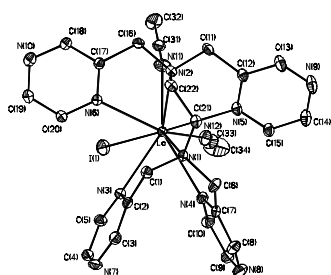
Fig.2 Crystal structure of the cation [La(tpzen)(MeCN)_2]^{2+} in 2 , with thermal ellipsoids at 30 % probability. Selected bond lengths (Å): La-N(1) 2.734(3), La-N(2) 2.698(3), La-N(3) 2.748(3), La-N(4) 2.661(4), La-N(5) 2.704(4), La-N(6) 2.703(4), La-N(11) 2.650(4), La-N(12) 2.666(4), La-I(1) 3.2379(5).
