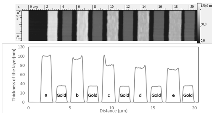
Figure 1. AFM image of gold electrodes grafted in different conditions with a TBPFd diazonium salt (up) and its corresponding profile (down). The electrodes a, b, c, d and e are grafted while the gold electrodes are used as a height reference.
