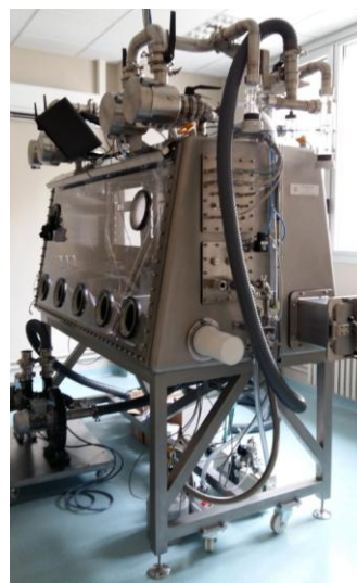
Figure 2. The TAP glove box
