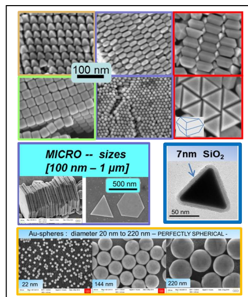
Figure 1: Illustration of some of our monodisperse gold nano-particles, micro-plates and hybrids (Au@SiO 2 ) with tunable sizes and thicknesses.
