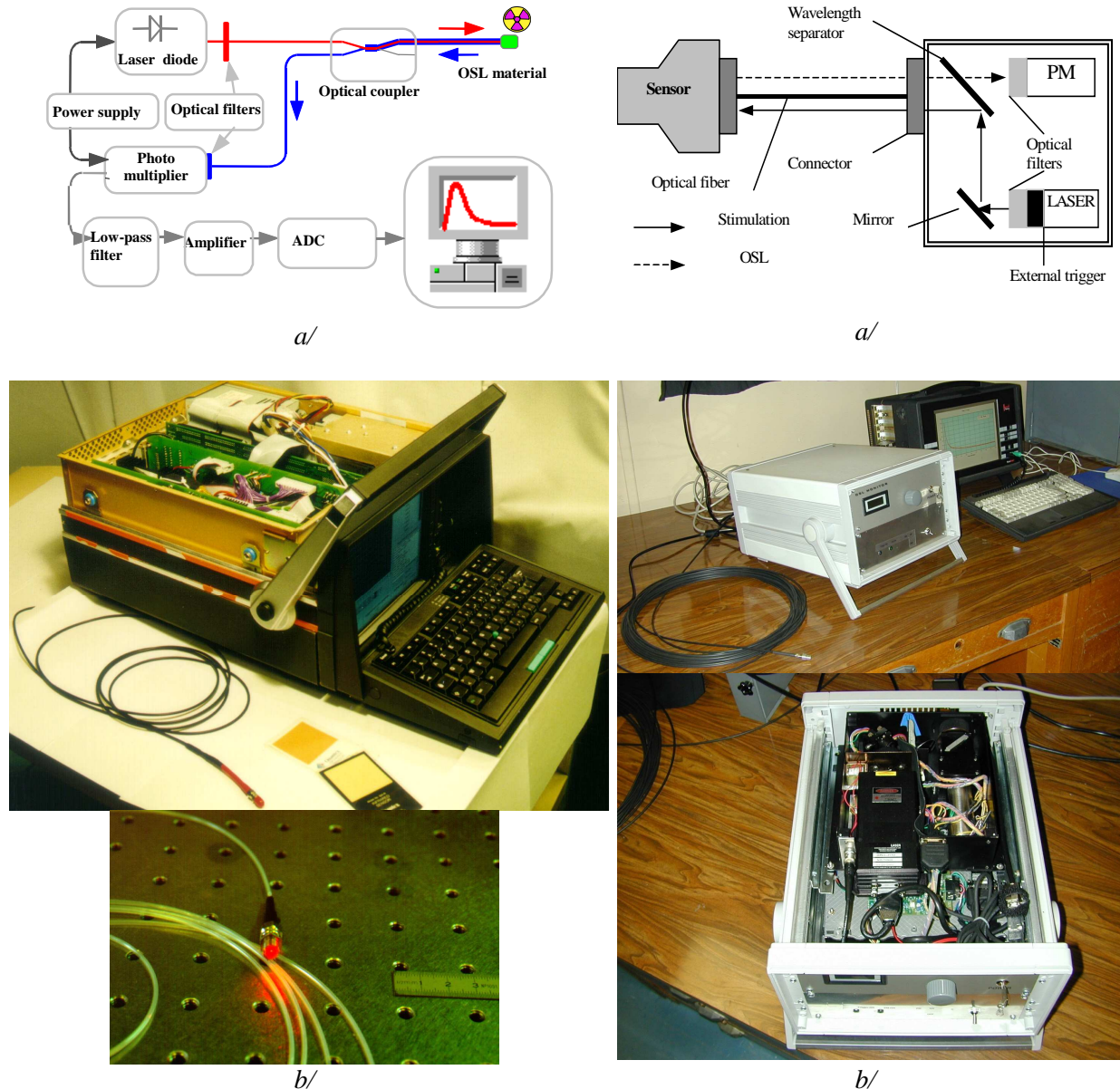
FIG. 2 : First generation of OSL optoelectronic dosimeters (OSL 1) a/ OSL 1 : Scheme of operation b/ View of the PC-based system and fiber-connected OSL transducer
