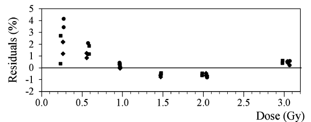
Fig. 6. (Top) Evolution of the integrals of OSL signals for OSL#3 (TLD 500 ) for the three reference energies (6 MV, 12 MV, and 20 MV). (Bottom) Relative difference (residuals) between OSL data and each fit equation associated to each reference energy.
