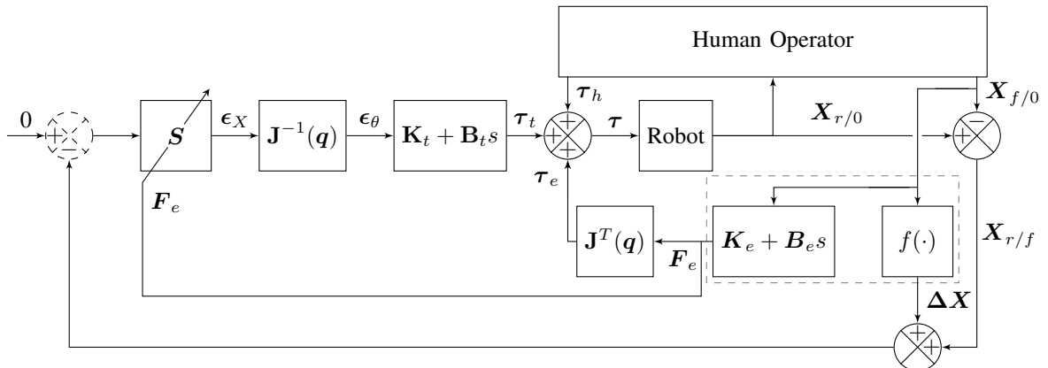
Fig. 3. Control law with switch, in the framework of [11]. S: Switch, see (3). Dashed area: Virtual Environment. f(\cdot) : tracking compensation, see (4).
