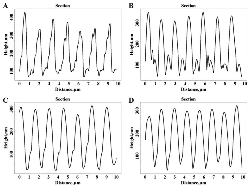
Figure 6. AFM images (cross sections) of the SRGs corresponding to sample 3 obtained with 200 pulses and different fluence values: (A) 4.3, (B) 8.8, (C) 14.2, and (D) 16.5 \text{ mJ/cm}^2 . The film thickness was 500 nm, and the SRG periodicity was 1.4 \mu\text{m} .
