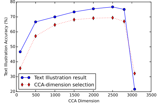
Figure 1: CCA_{cap} result and dimension selection
