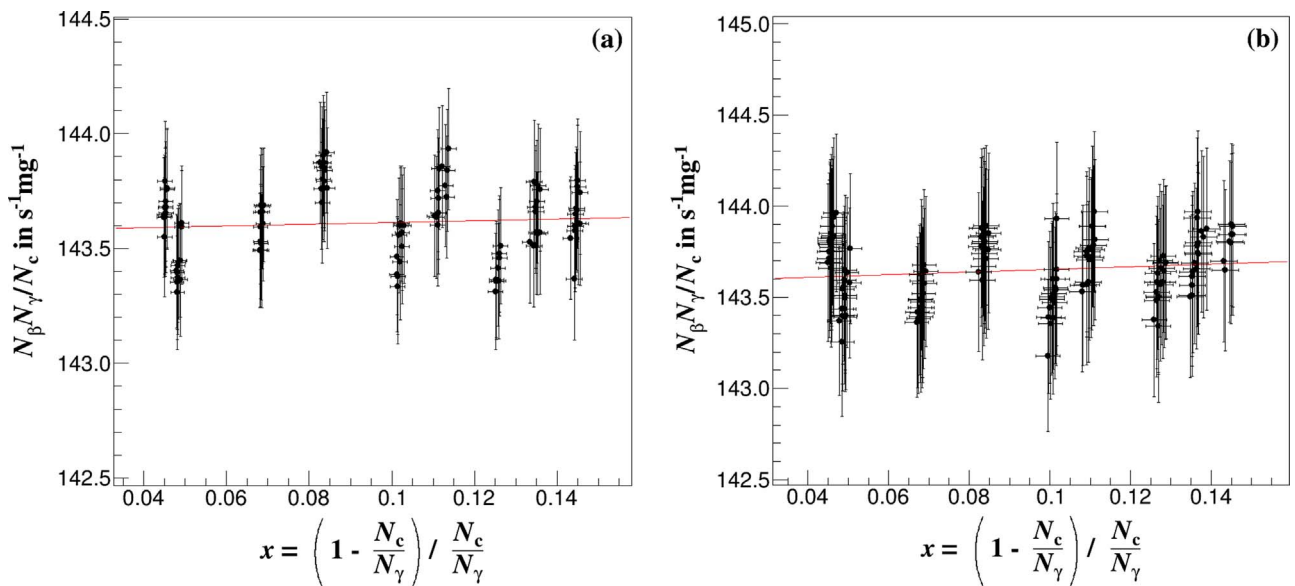
Fig. 4. \frac{N_{\beta} \cdot N_{\gamma}}{N_c} measured with a 4\pi\beta(\text{PC})-\gamma coincidence system as a function of x = \frac{\left(1 - \frac{N_c}{N_{\gamma}}\right)}{\left(\frac{N_c}{N_{\gamma}}\right)} ; function f(x) is a 1st degree polynomial which was fitted to the experimental data, and the bars represent the statistical uncertainty of the individual data. In the left figure an open \gamma window was used, whereas the \gamma window was limited to the region of the two dominant peaks at 1173 keV and 1332.5 keV in the right figure.
