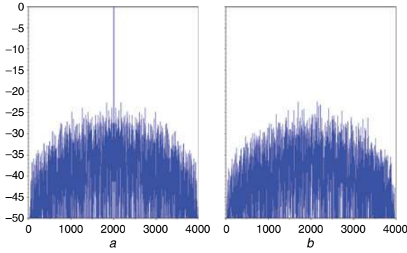
Fig. 1 a Auto-correlation b Cross-correlation of two chaotic signals, using N=10 , M=200 , k_1=3.9 and k_2=3.900001 , and random initial conditions x_0
