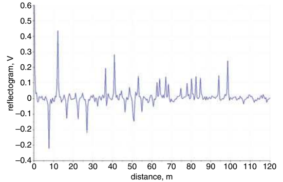
Fig. 3 Reflectogram from point A. CTDR signal's parameters: N=50 , M=200 , k=3.9
