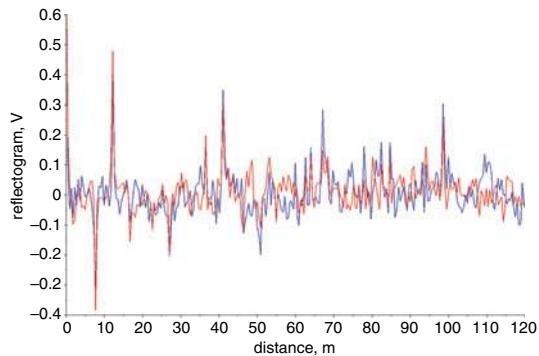
Fig. 5 Reflectogram from point A, with 10 (red curves) and 20 (blue curves) random emitting sensors
