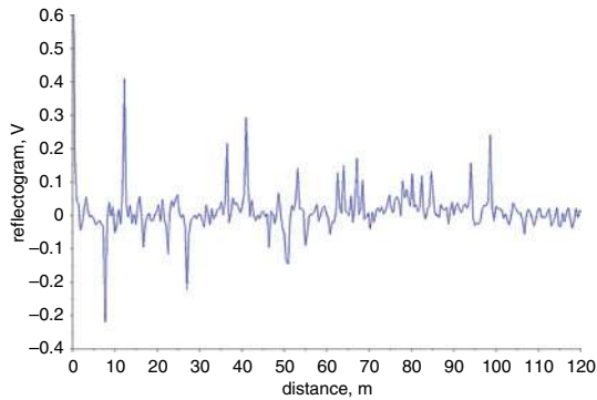
Fig. 4 Reflectogram from point A, with four emitting sensors at points C, E, G and H. CTDR signal's parameters: N=50 , M=200 , k=3.9 + \text{rand}(0,1)/100
