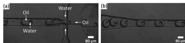
Fig. 8 Formation of W/O/W emulsions in a chip plasmated five days before and stored at -18 \text{ }^{\circ}\text{C} before use. (a) Formation of water-in-oil-in-water droplets at the second junction, (b) no wetting of the oil droplets was observed.
