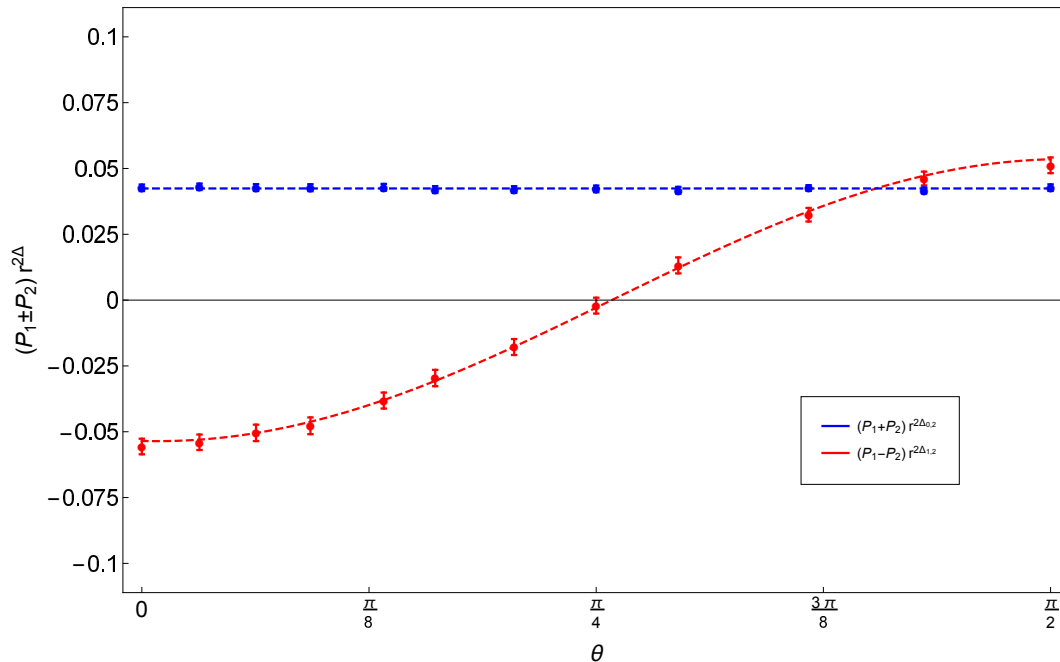
Figure 4. Linear combination P = P_1 \pm P_2 , where P_1 = \mathbb{P} \begin{pmatrix} | \\ | \end{pmatrix} and P_2 = \mathbb{P} \begin{pmatrix} \times \\ \times \end{pmatrix} , of renormalised probabilities for the propagation of N = 2 clusters in percolation ( Q = 1 , or x = 2 ). A rotations corresponding to the one described on the right panel of Figure 3 is performed and parametrized by \theta . The red plot corresponds to (3.3) and the blue plot to (3.5), whose angular dependence is proportional to 1 and \cos 2\theta , respectively.
