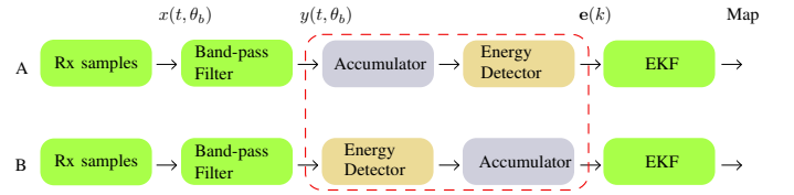
Fig. 4. Receiver schemes.
