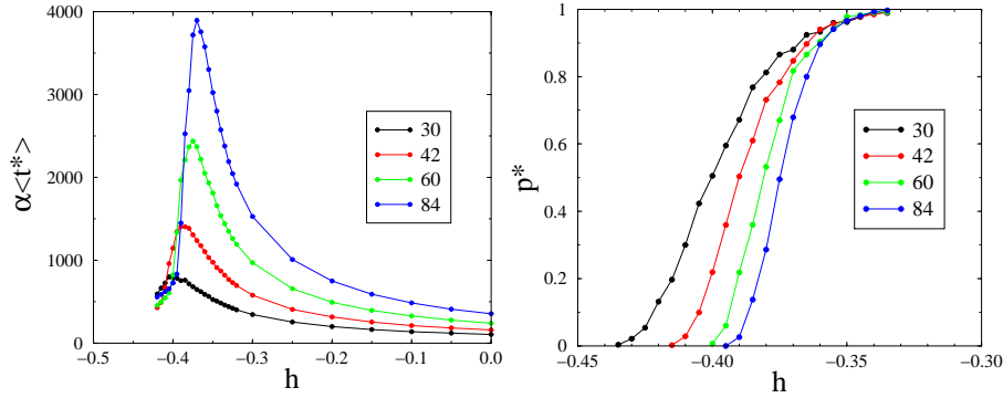
Figure 14. Mean stopping time \alpha \langle t^* \rangle (left) and splitting probability p^* (right), against magnetic field h for T/T_c = 0.5 . Symbol colors denote values of N .
