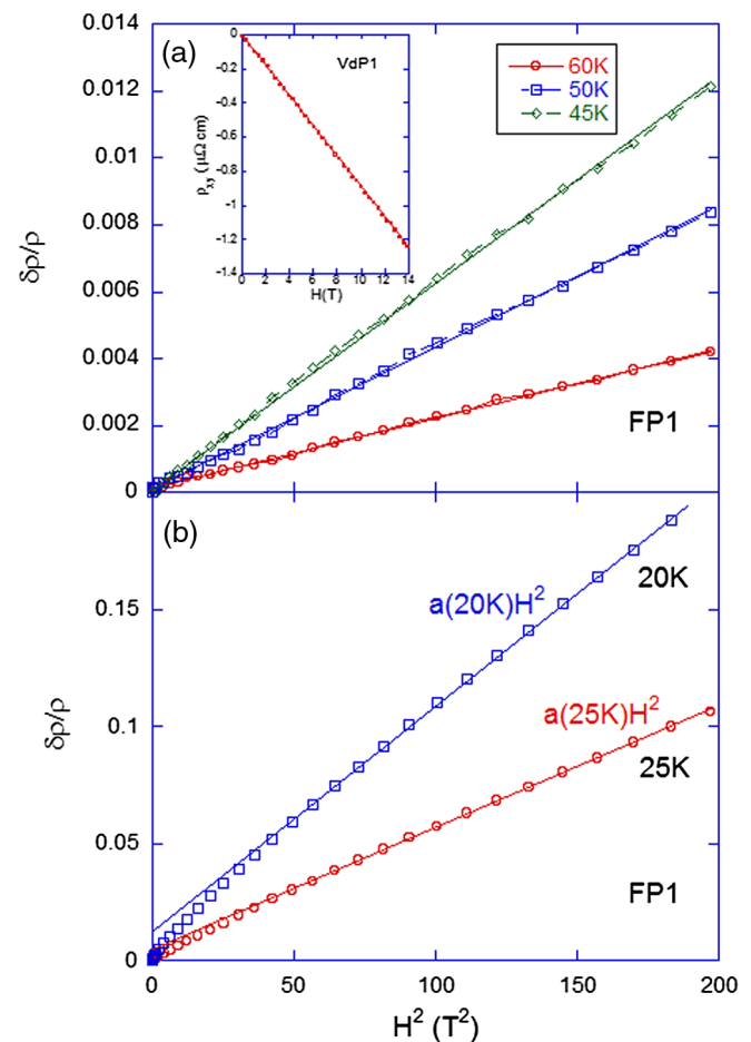
FIG. 1 (color online). (a) Magnetoresistance curves versus H^2 at 45, 50, and 60 K for sample FP1. Straight lines are linear fits of the data. The inset shows the Hall effect data for sample VdP1 at 60 K for magnetic fields up to 14 T. The straight line is a linear fit of the data. (b) Magnetoresistance curves versus H^2 at 20 and 25 K. Straight lines are linear fits of the data at high magnetic fields.
