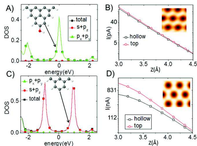
Figure 11. (A) Electronic DOS of the O atom when an OH group replaces the last H atom in the graphitic tip as shown in the inset. Black squares represent the total DOS of the oxygen apex, red circles are the s + p_z orbitals and green up triangles correspond to the p_x + p_y orbitals. (B) I(Z) curves calculated over a C atom (red circles) and a hollow position (black squares) including the MS effects. In the inset, the resulting STM image with the honeycomb pattern is shown. (C) and (D) the same for the graphitic tip when the last H atom is removed. The voltage applied in this case is -1.0 V.
