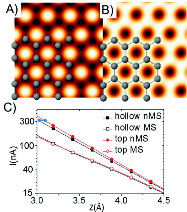
Figure 5. Calculated STM images obtained with our gold tip: (A) triangular pattern with the maxima over the hollow positions obtained at 3.0 Å and (B) honeycomb pattern and atomic resolution at 4.5 Å. (C) I(Z) curves calculated over a C atom (red circles) and a hollow position (black squares) with/without the inclusion of the MS effects (open/filled symbols). The change between the hexagonal and triangular regime is produced at a tip–sample distance of 3.35 Å. The blue line defines the way the corrugation is estimated. The WSxM software has been used to plot the STM images [40].
